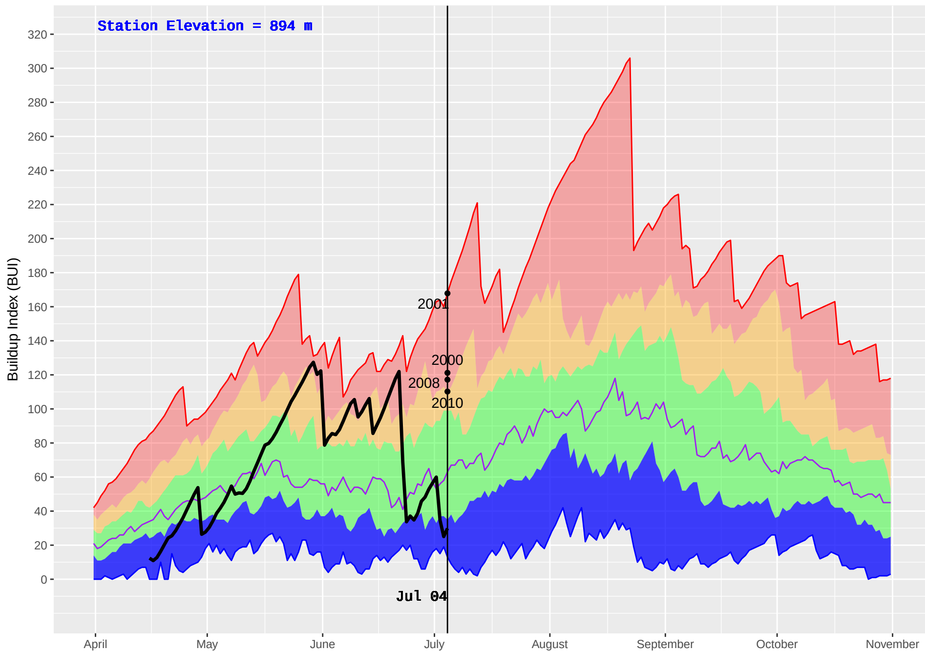
TOBY HUB (417) : Historical (1986–2016) and Current (2018) Noon Buildup Index (BUI)
