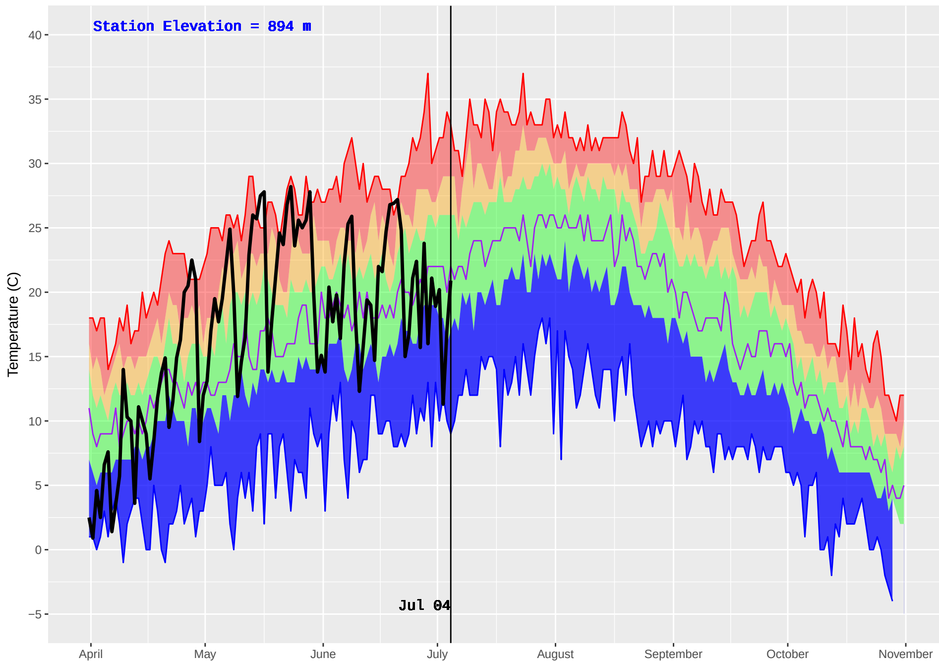
TOBY HUB (417) : Historical (1986–2016) and Current (2018) Noon Temperature
